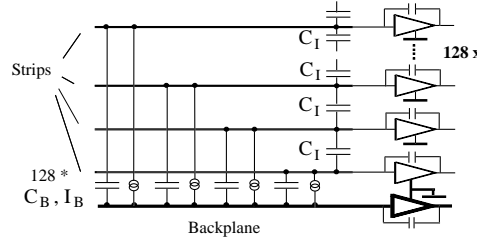
Figure 5: Capacitance network for the readout system. The following numbers are estimated for the SVX. Typical values for 300 \text{ } \mu\text{m} strip detectors are in brackets:
