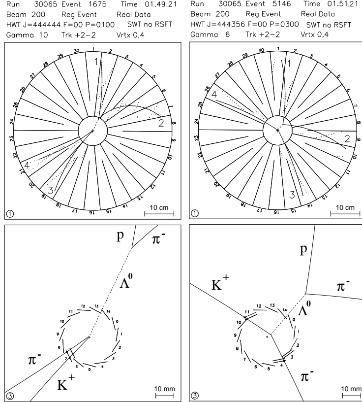
Figure 3: r\phi projection of the charged tracks of two events with a \Lambda decaying in p\pi^- , recorded from \bar{p} annihilations in liquid deuterium.
