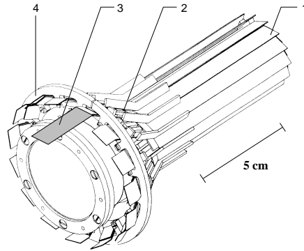
Figure 1: 3 D view of the Si-vertex-detector. 1: Si- \mu -strip detectors, 2: Hybrid, 3: Electronics and flat band cables, 4: Cooling ring.
