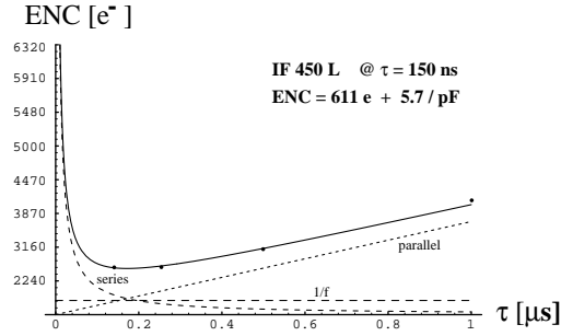
Figure 6: backplane noise versus shaping time in number of electrons rms.
